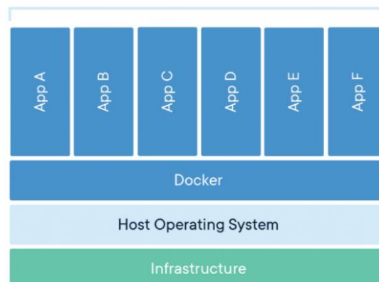
Containerized Applications
